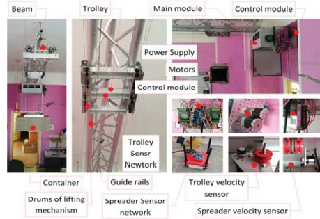
Fig. 2. Experimental test-bed [20].
