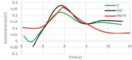
Fig. 5. Experimental results – extremums of cargo oscillation (S-control using “S” shaped velocity profile only, PID – control using PID with “S”-shaped velocity profile, PID PI – control using full developed algorithm with compensation feedback).
