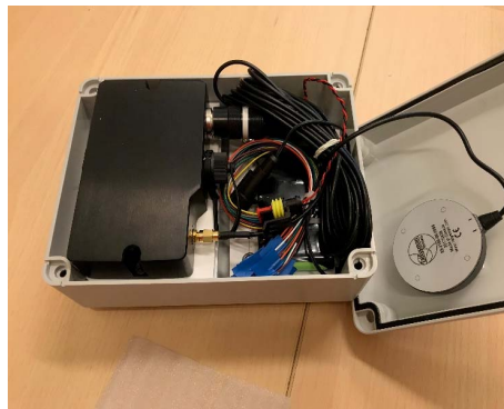
Fig. 1. Secured case with DL-1 MK2 Data logger, GPS antenna and additional connector for output connections.
