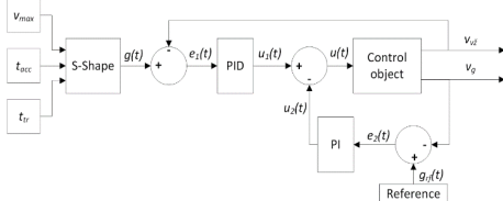
Fig. 1. General block diagram of control system.
