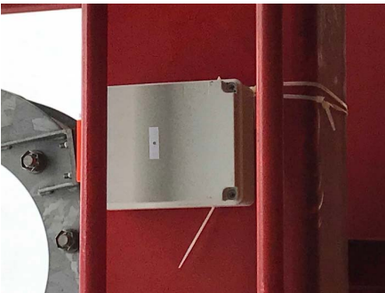
Fig. 3. Demonstration of the Data Acquisition sensory hardware placement on the crane spreader with details of its placement and mounting equipment.
