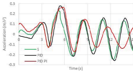
Fig. 4. Experimental results – cargo oscillation (S-control using „S“ shaped velocity profile only, PID – control using PID with „S“-shaped velocity profile, PID PI – control using full developed algorithm with compensation feedback).
