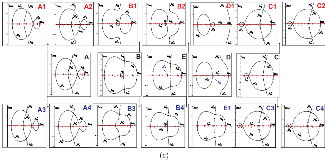
Fig. 1.20. The trajectories of the third order and the second order Critical points and Spectrum Curves, A = (0.3526\dots, 0.8560\dots) , B = (0, 3600\dots, 0.8601\dots) , C = (0.4491\dots, 0.8771\dots) , D = (0.3660\dots, 0.8660\dots) , E = (0.3603\dots, 0.8603\dots) .
